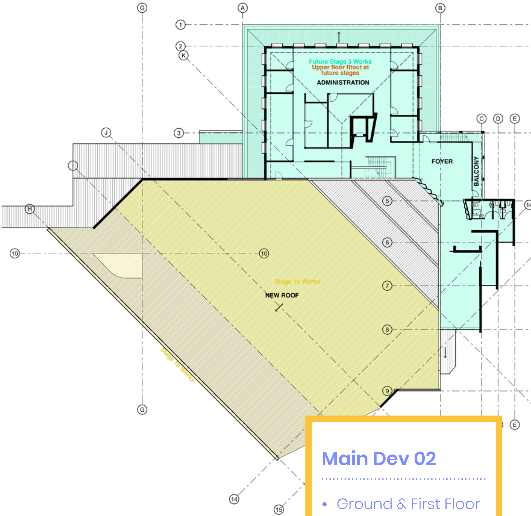
02 First Floor Staging Plan 1:200
