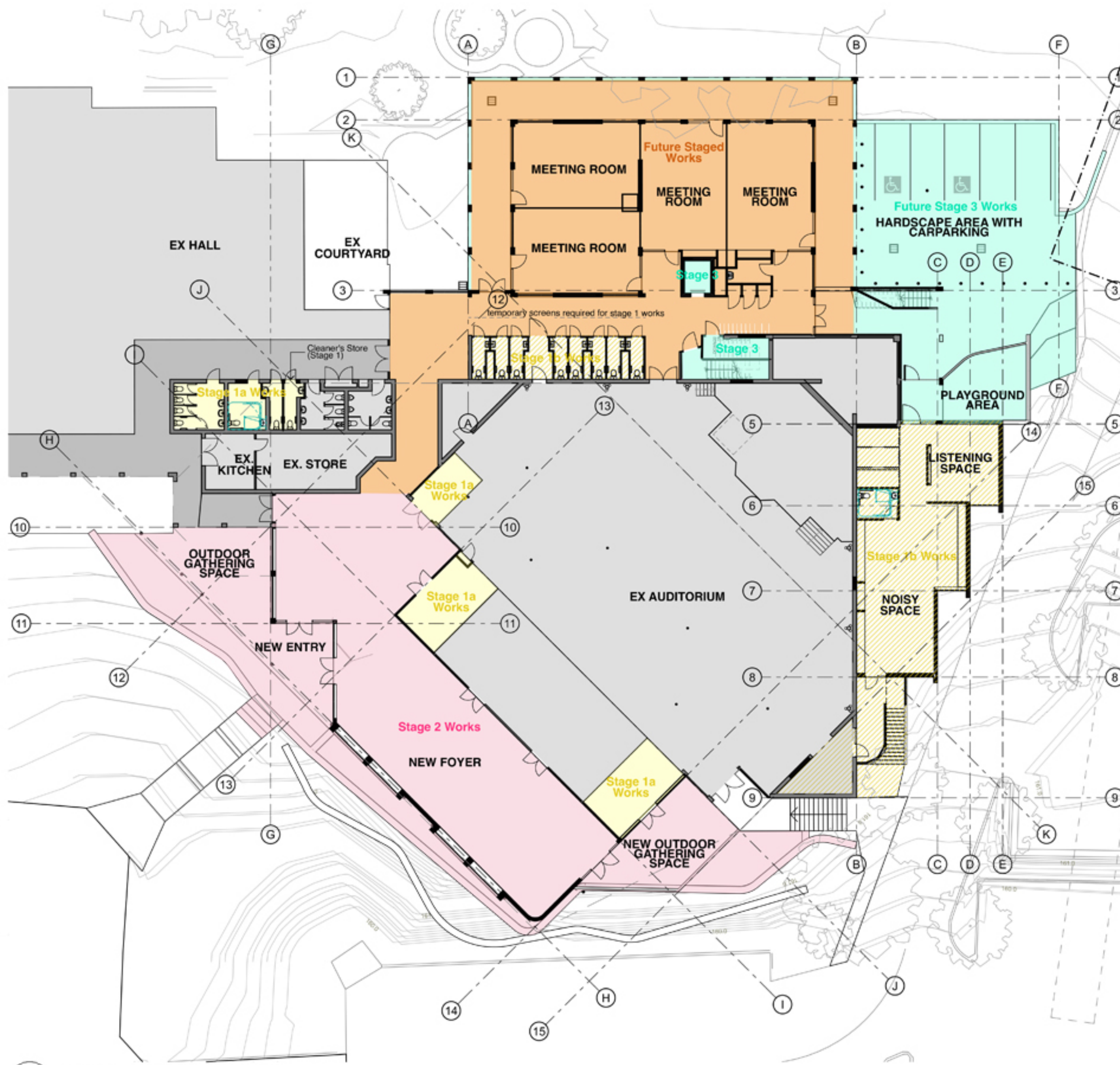
01 Ground Floor Staging Plan 1:200
